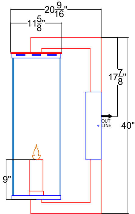
MEDIUM B-026-012 11 \frac{5}{8} "W x 40"H x 20 \frac{9}{16} "D
