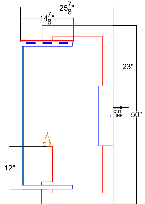
XLARGE B-026-014 14 \frac{7}{8} "W x 50"H x 25 \frac{7}{8} "D
