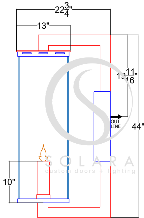
LARGE B-026-013 13"W x 44"H x 22 \frac{3}{4} "D
